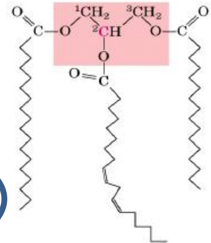
1-Stearoyl, 2-linoleoyl, 3-palmitoyl glycerol, a mixed triacylglycerol
